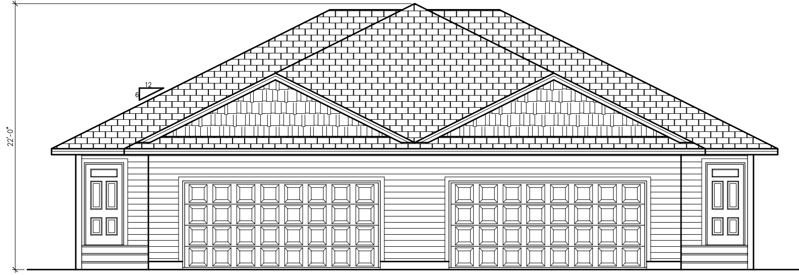
FRONT ELEVATION 1/4"=1'-0"
