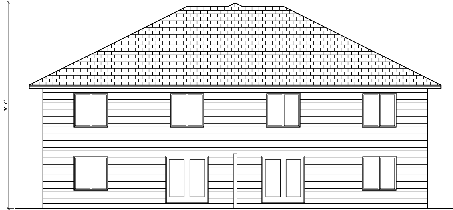
REAR ELEVATION 1/4"=1'-0"
